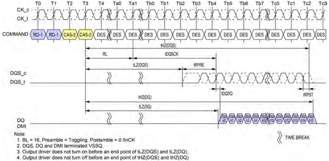
Figure 11 - Read Timing
