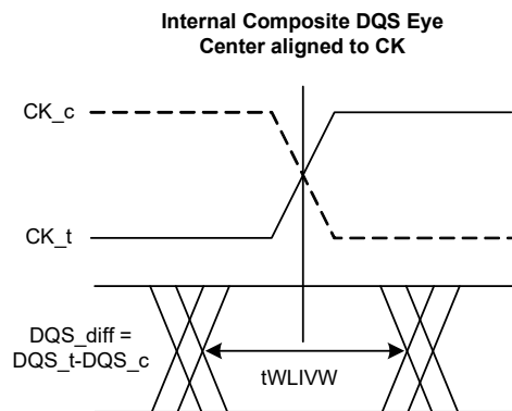
Figure 117 - DQS t /DQS c and CK t /CK c at DRAM Latch
