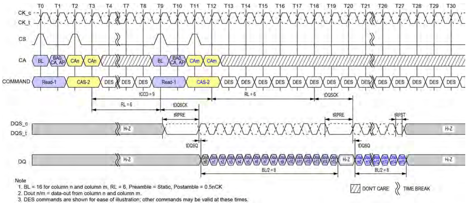
Figure 33 - Consecutive Reads Operation: t_{CCD} = \text{Min} + 1 , Preamble = Static, 0.5nCK Postamble
