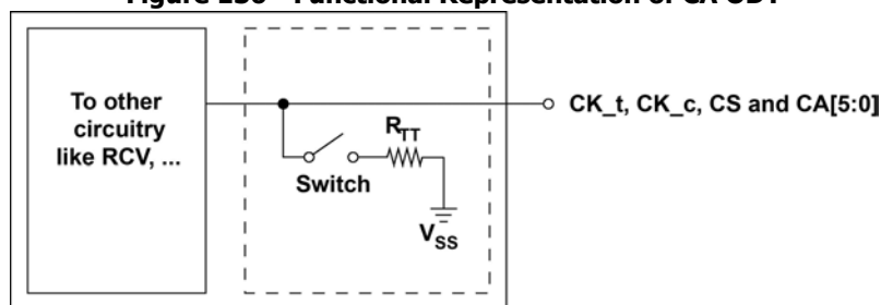
Figure 136 - Functional Representation of CA ODT
