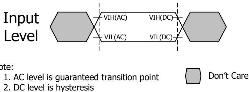
Figure 168 - Input AC timing definition for CKE
