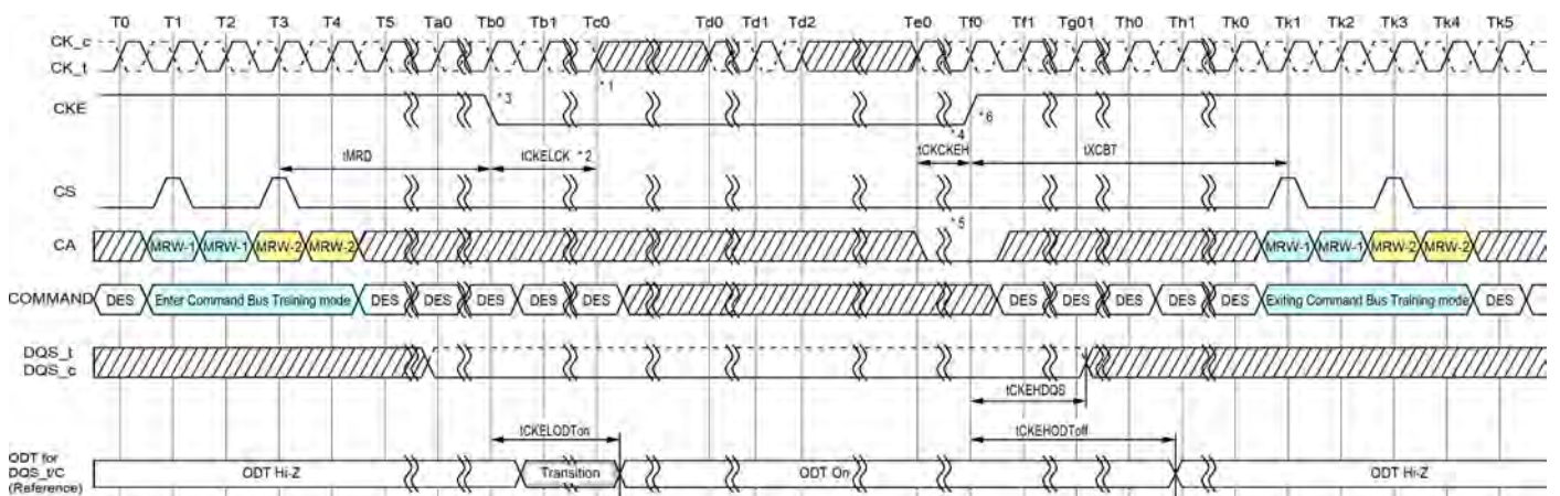
Figure 108 - Exiting Command Bus Training Mode
