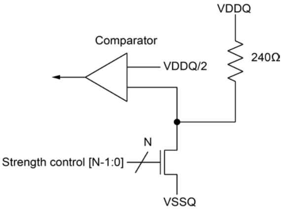
Figure 186 - Pull-down calibration
