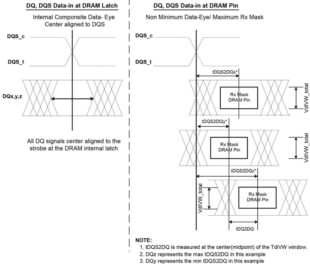
Figure 197 - DQ to DQS ( t_{DQS2DQ} and t_{DQDQ} ) Timings at the DRAM pins referenced from the internal latch
