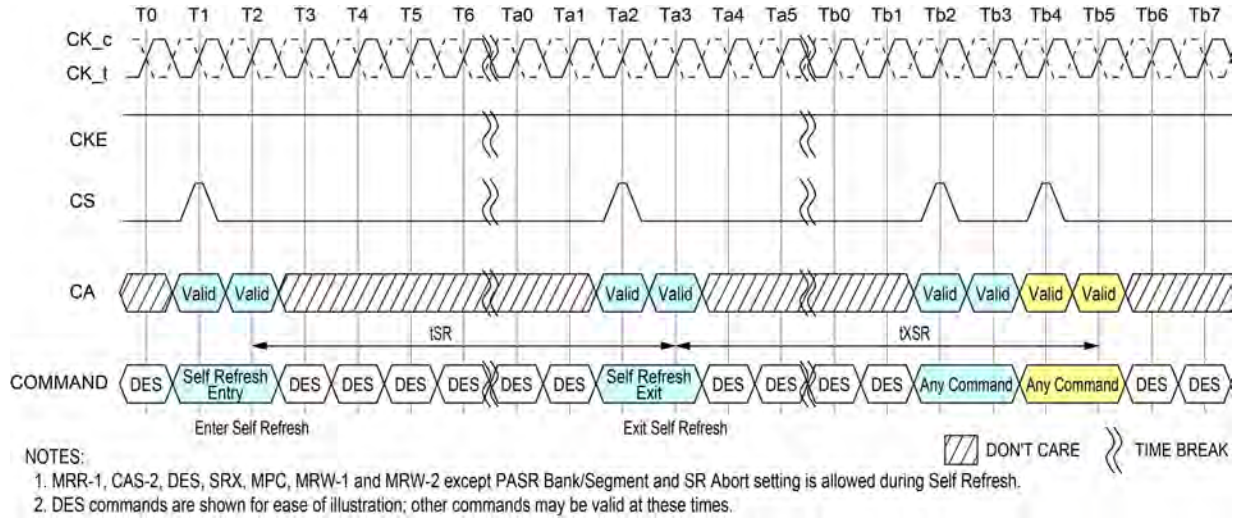
Figure 71 - Self Refresh Entry/Exit Timing
