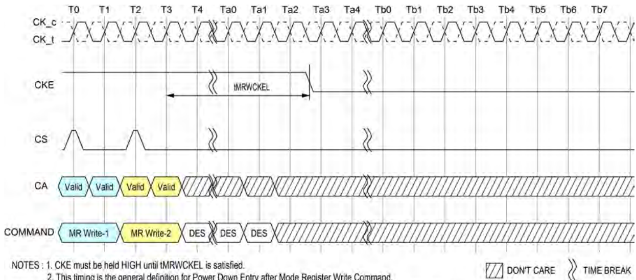
Figure 163 - MRW to Power-Down Entry
