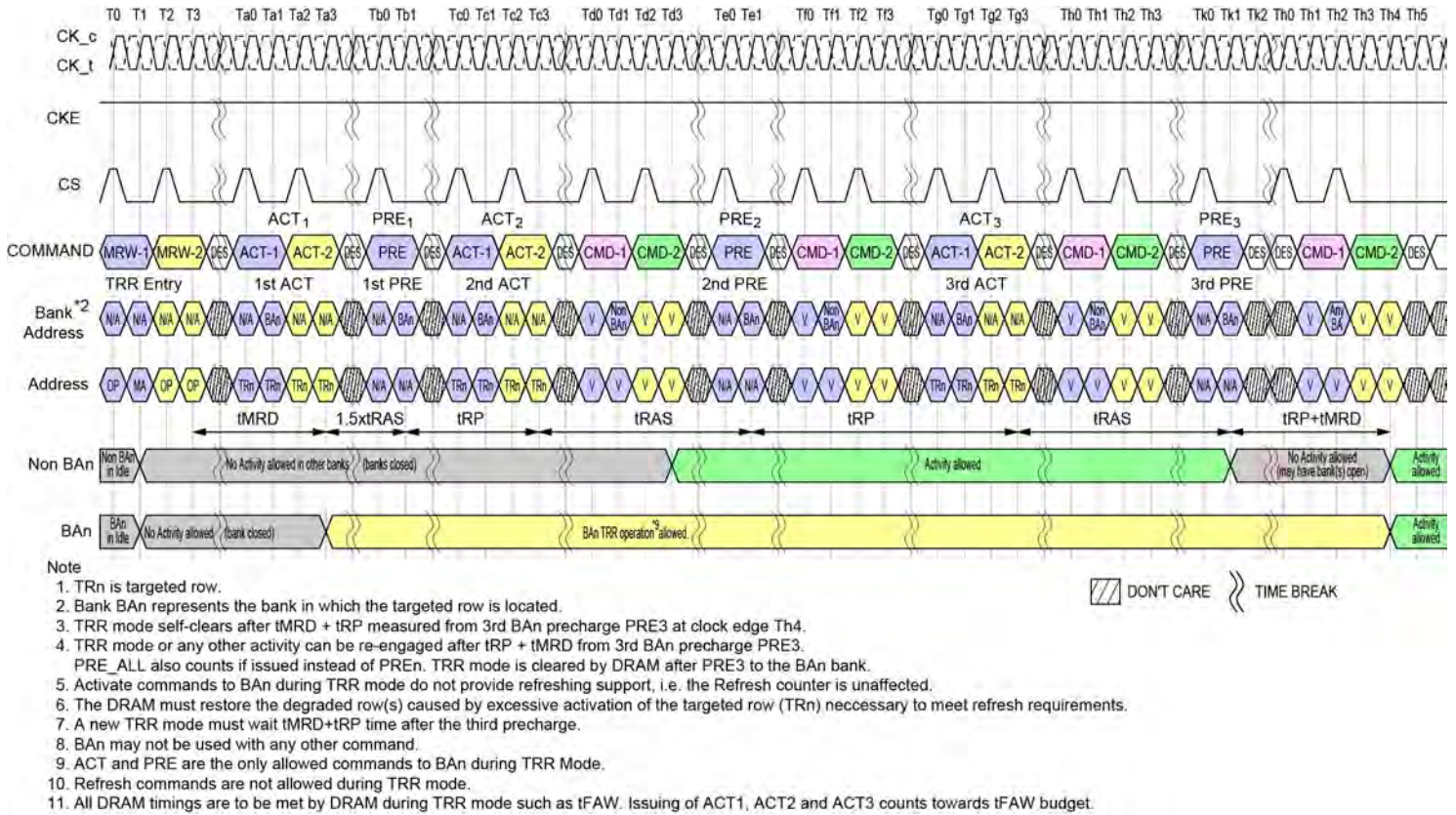
Figure 166 - TRR Mode Timing Example
