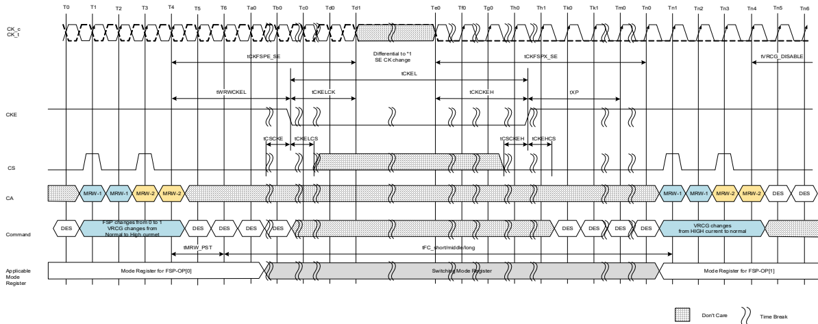
Figure 146 - Differential to SE CK and Write DQS -FSP Switching Timing CKE=Low
