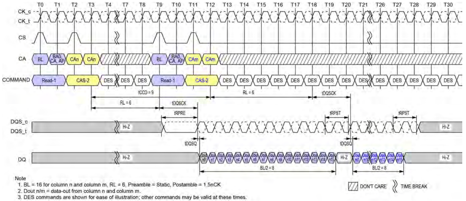
Figure 32 - Consecutive Reads Operation: t_{CCD} = \text{Min} + 1 , Preamble = Static, 1.5nCK Postamble
