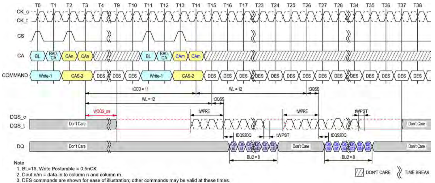
Figure 49 - Consecutive Writes Operation: t_{CCD} = \text{Min} + 3, 0.5n\text{CK} Postamble
